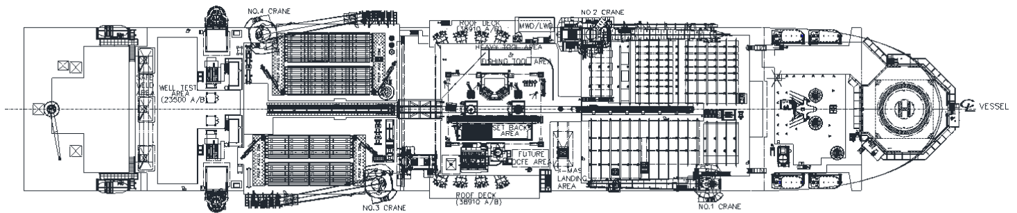
DRILL FLOOR & PLAN
